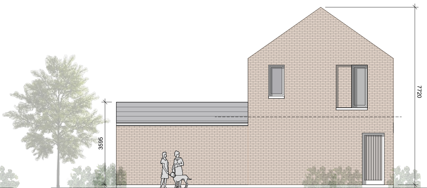
GABLE ELEVATION
